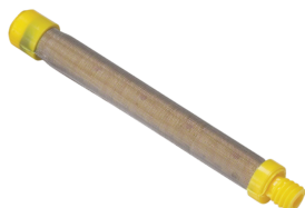
TT0003852 Filtru Galben fin, mesh 100, maner pistol, filet stanga
